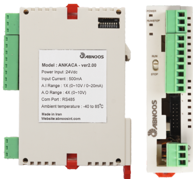
Analog Input / Output Card
