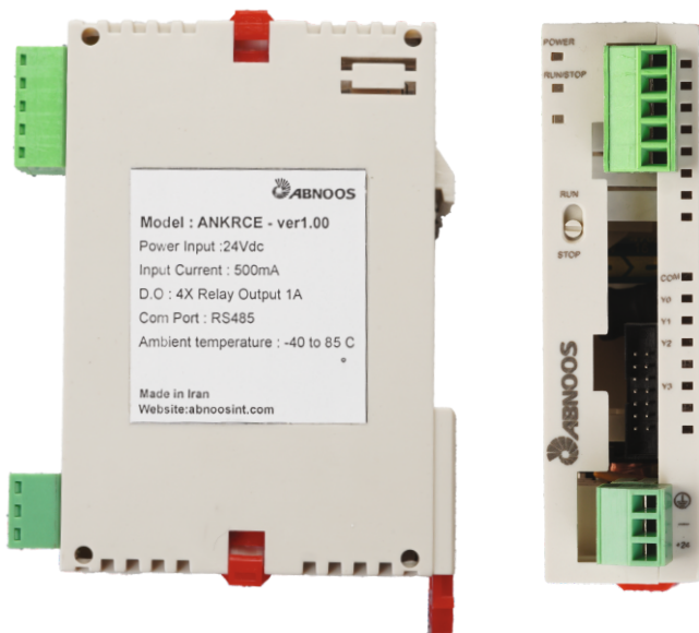
SMS Module Relay Card
